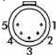
DMX 512 Connector XLR-5p connector
